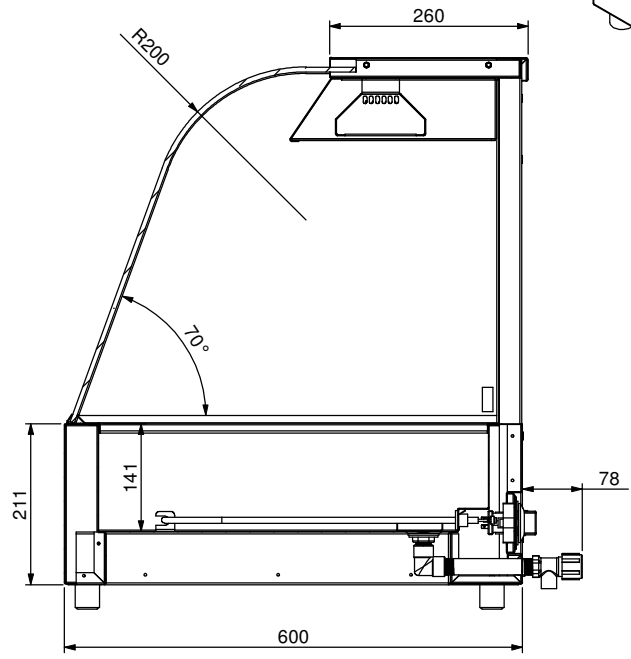
SECTION H-H
