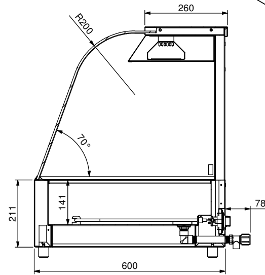
SECTION F-F
