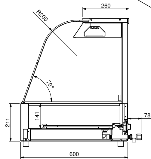
SECTION F-F
