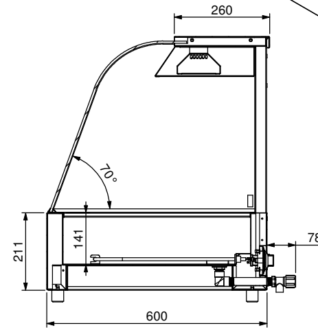
SECTION F-F
