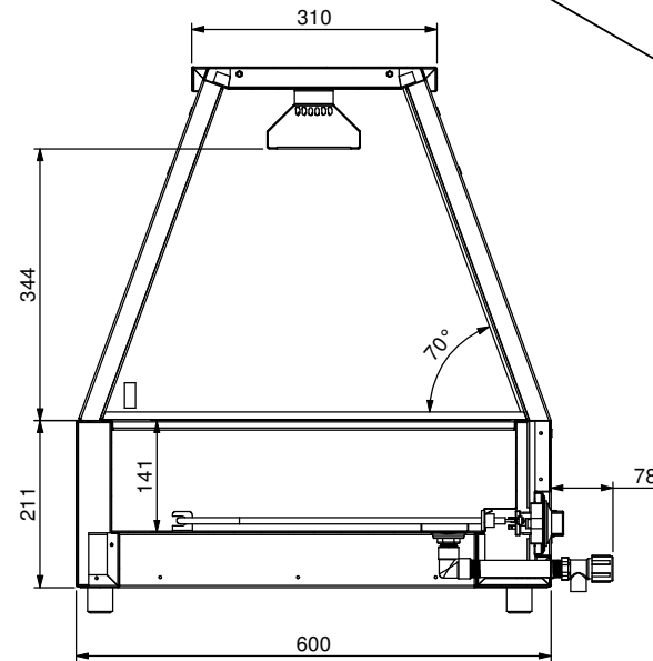
SECTION S-S
