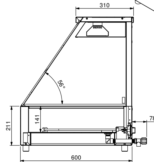
SECTION CF-CF
