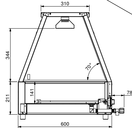
SECTION R-R
