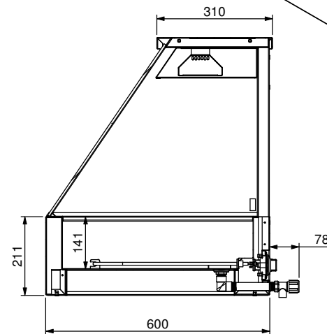
SECTION ED-ED
